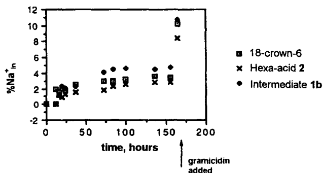
Figure 4. Plots of growth of \text{Na}_{\text{in}}^+ over time resulting from the presence of 18-crown-6, hexaacid 2 , and fully protected channel 1b in vesicles, at concentrations of 1.0 mol%.
