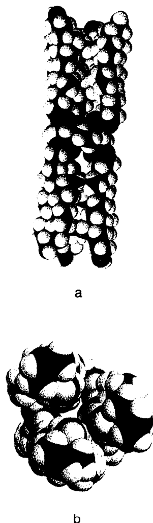
Figure 2. Space-filled model of the ion channel: (a) Long view; (b) top view, as generated from MacroModel.
